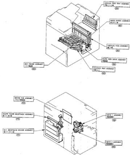
FIGURE A ASSEMBLY LOCATION DIAGRAM (3/5) 主要部品配置図 (3/5)
